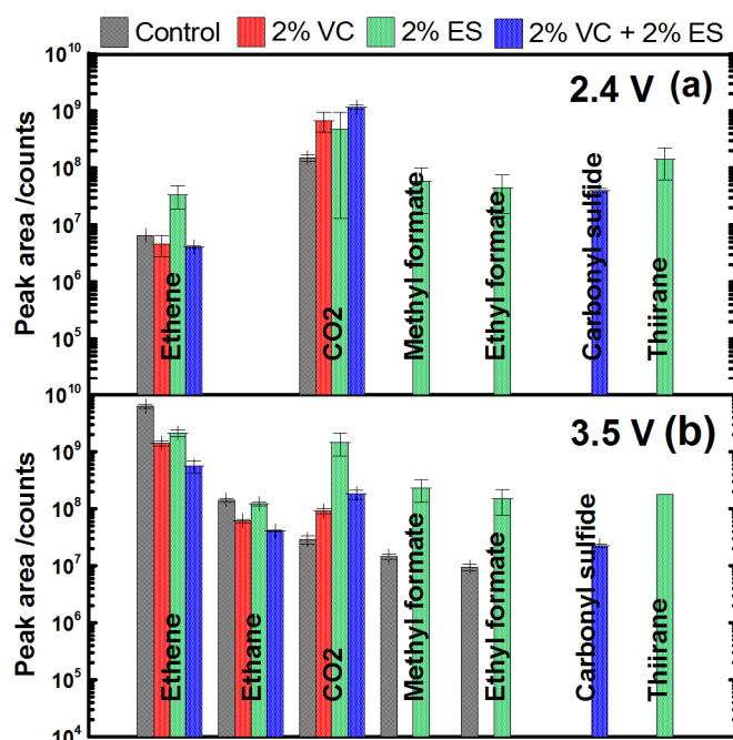
Figure 5. GC-MS data for the primary gases extracted from NMC/graphite pouch cells for the different electrolytes after formation at (a) 2.4 V and (b) 3.5 V. The data presented here shows the normalized peak area for compounds that are gaseous at room temperature.
