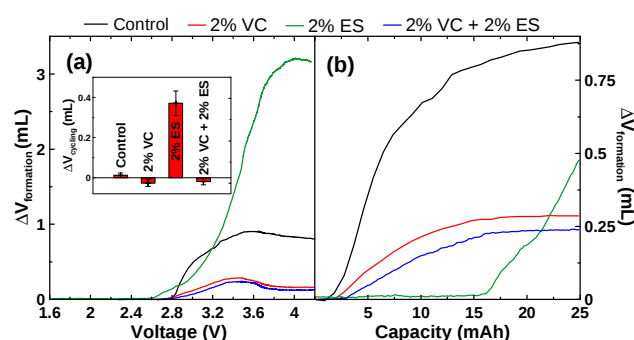
Figure 4. (a) Gas volume versus cell voltage (V) during the first charge of the formation cycle for NMC/graphite pouch cells containing different electrolytes; (b) gas volume versus capacity during the first 25 mAh of the formation cycle. Inset of figure 4a: Volume of gas evolved during the UHPC cycling at 11 mA (C/20) and 40.0 ± 0.1 °C for the NMC/graphite pouch cells containing the different electrolytes. A positive value means the cells are swelling while a small negative value indicates that the cell volume slightly shrinks.
