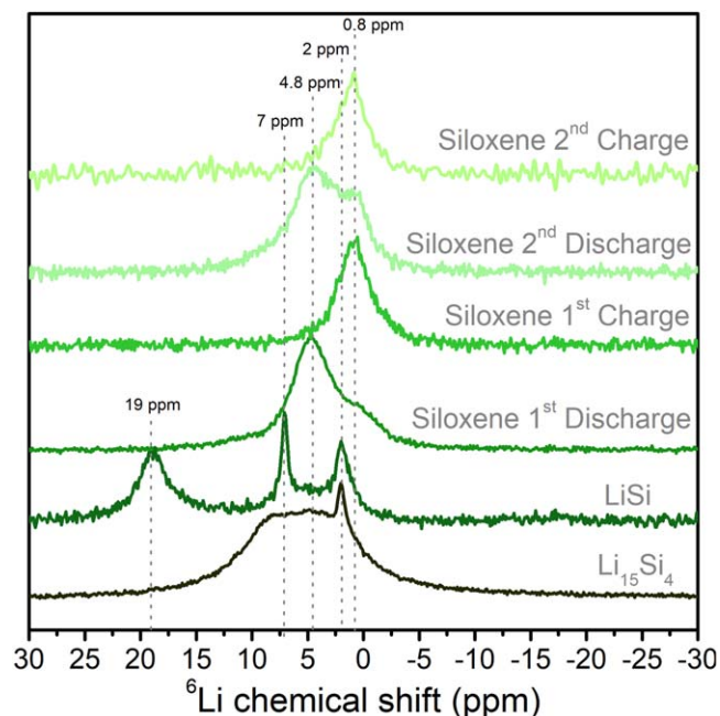
Figure 7. ^6\text{Li} NMR spectra of the 1st and 2nd lithiation/delithiation of a siloxene self-supported electrode and the LiSi and \text{Li}_{15}\text{Si}_4 references synthesized by ball milling.
